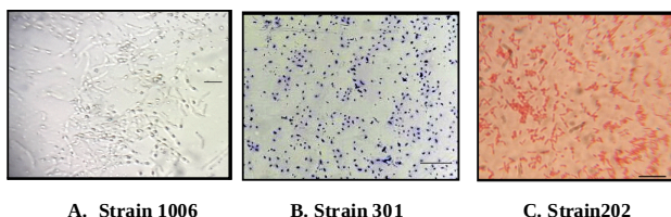
Fig. 3 : [A] Sporulating gram positive Bacilli type microorganism (Without stain) Strain 1006, tentatively identified as a strain of Bacillus from Singalila National Park (Phatak) [B]. Cocci type gram positive microorganism Strain 301, tentatively identified as strain of Micrococcus from Kalipokhari. [C]. Non-sporulating gram negative bacilli type microorganism Strain 202, tentatively identified as a strain of Pseudomonas from Tonglu. All scales represent 21m.
