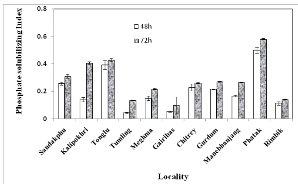
Fig. 2 : Phosphate solubilizing index* (after 48h and 72h) of the predominant phosphate solubilizing microorganism of the soil sample. *Phosphate solubilizing index = [Halo zone diameter (mm) - Colony diameter (mm)] / Colony diameter (mm) Culture was incubated at 30°C upto 72h.
